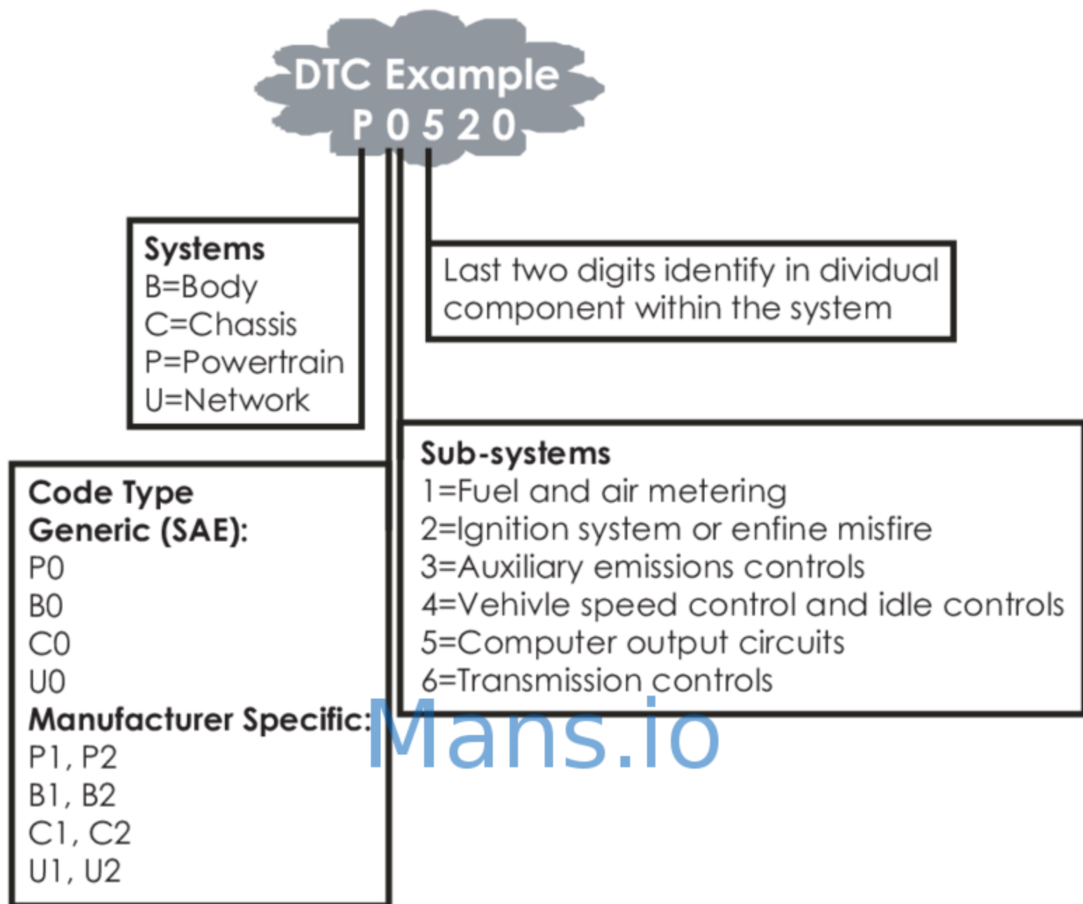
Figure 1-2: Explanation of a diagnostic trouble code.
