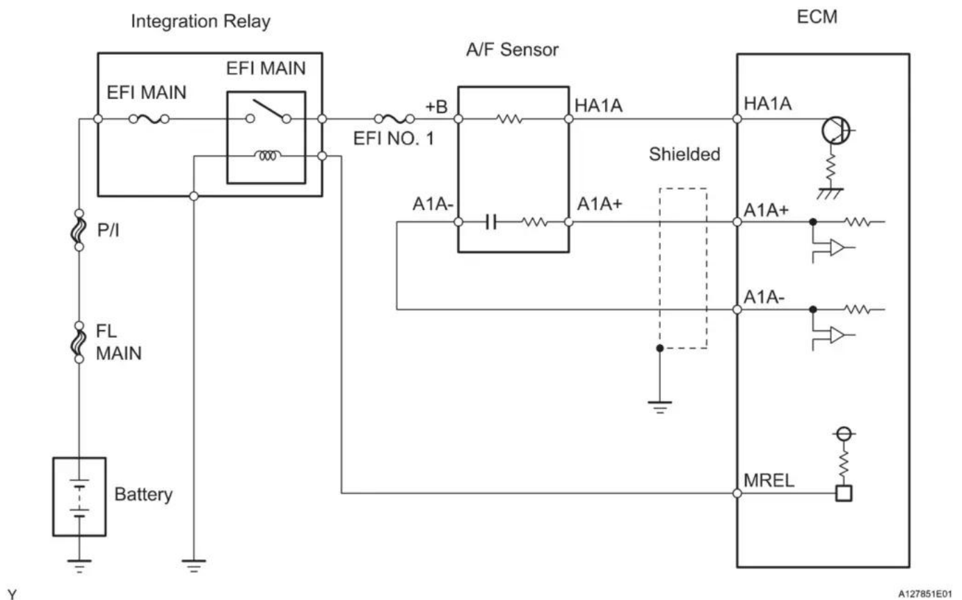
P2A00 wiring diagram
