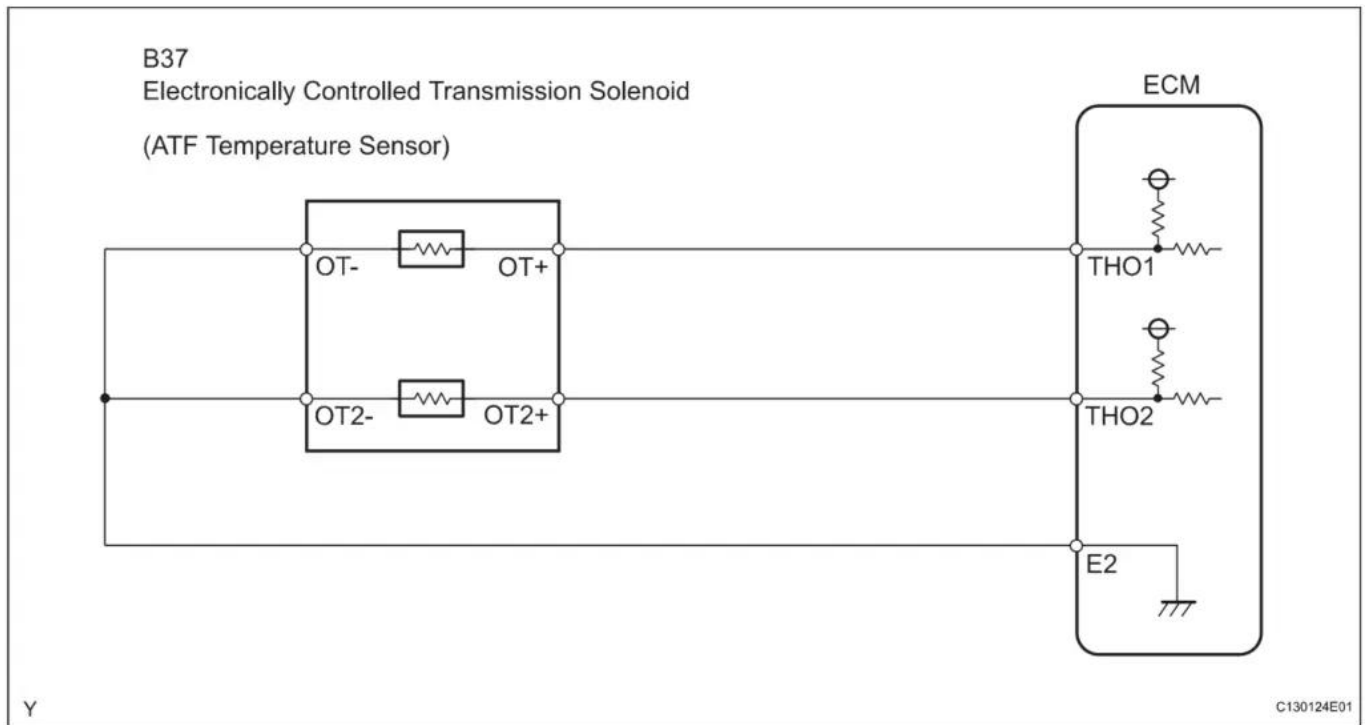
P2742 wiring diagram
