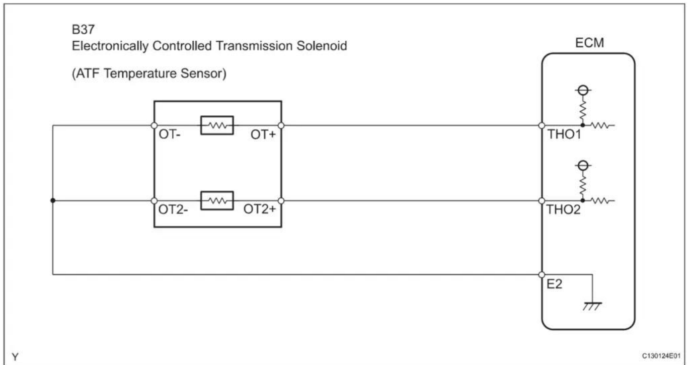
P2740 wiring diagram
