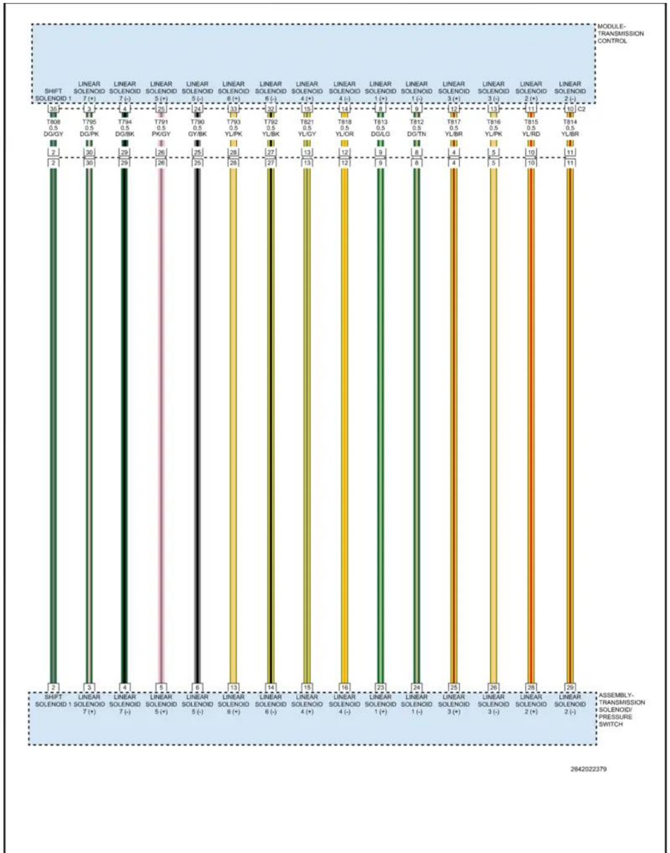
P2720 wiring diagram
