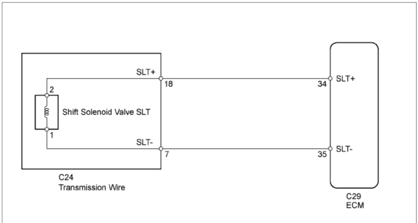
P2716 wiring diagram
