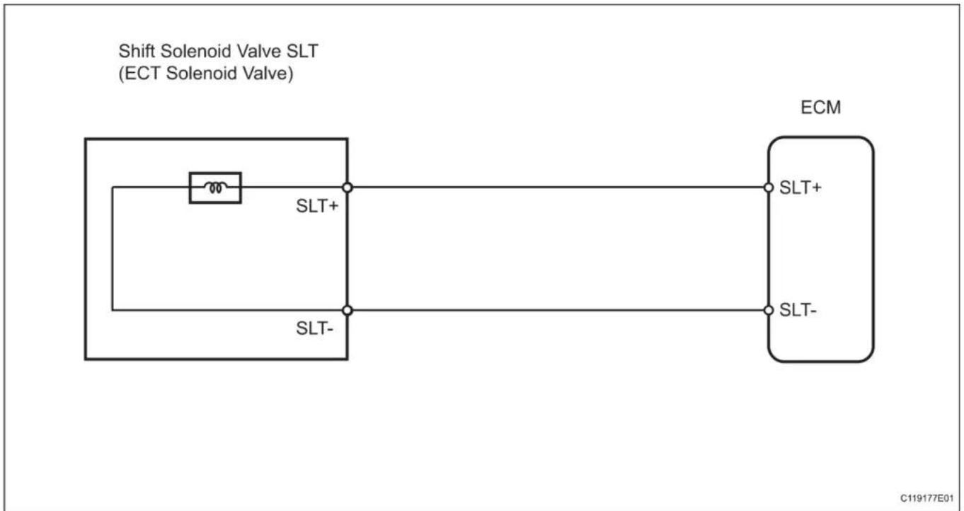
P2714 wiring diagram
