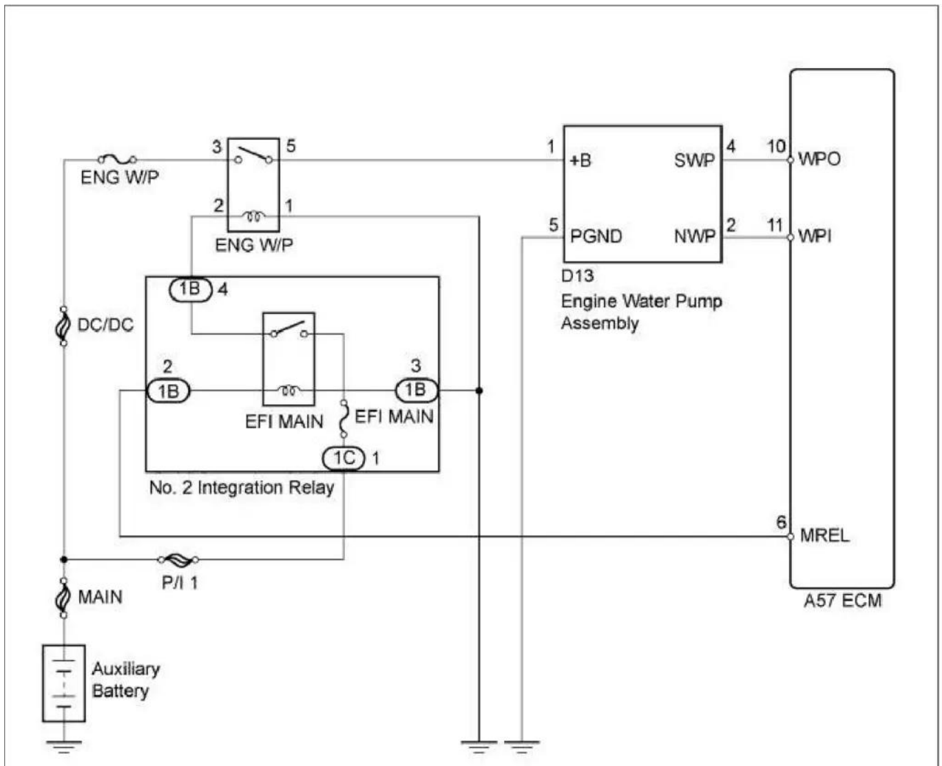
P261C wiring diagram
