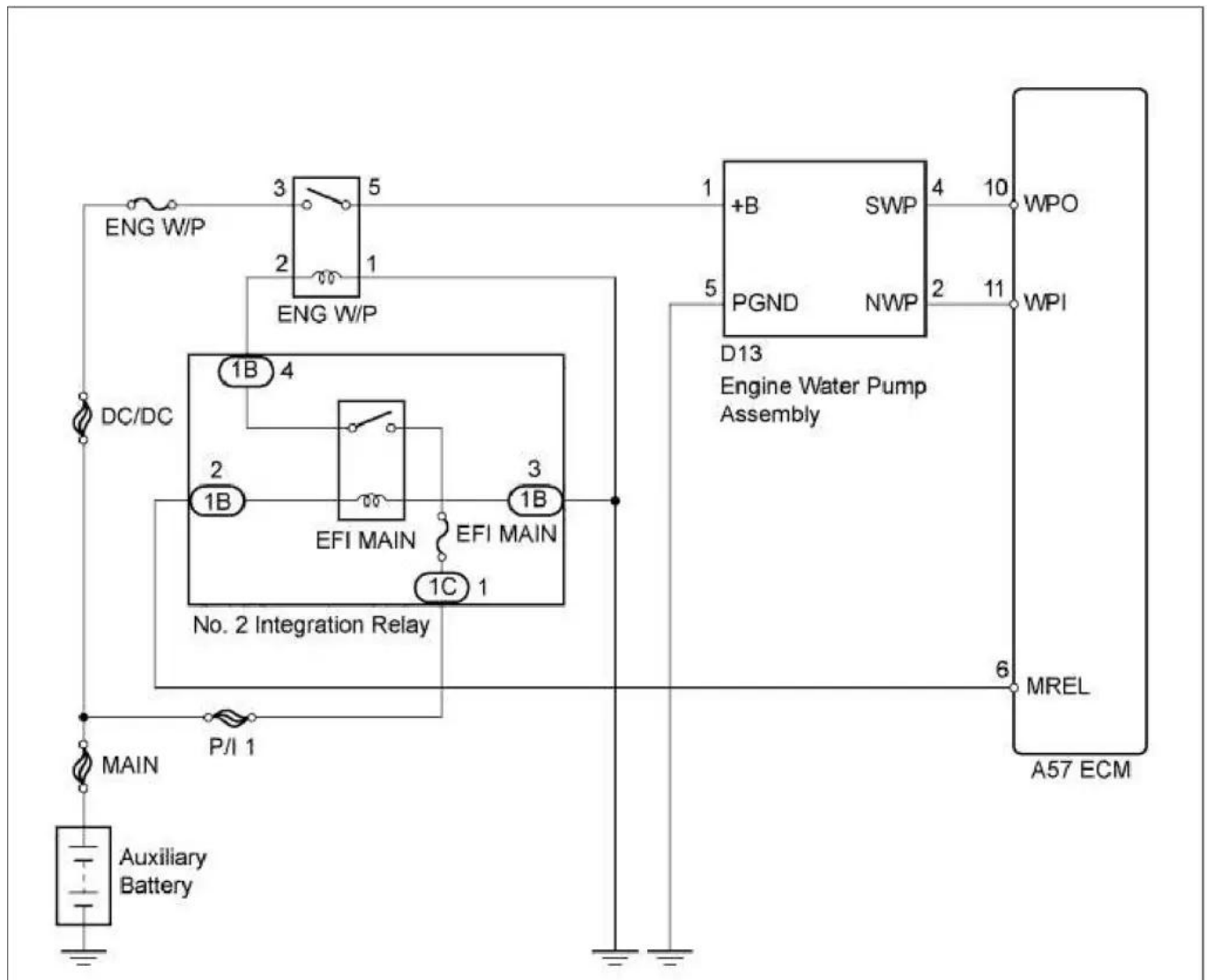
P261B wiring diagram
