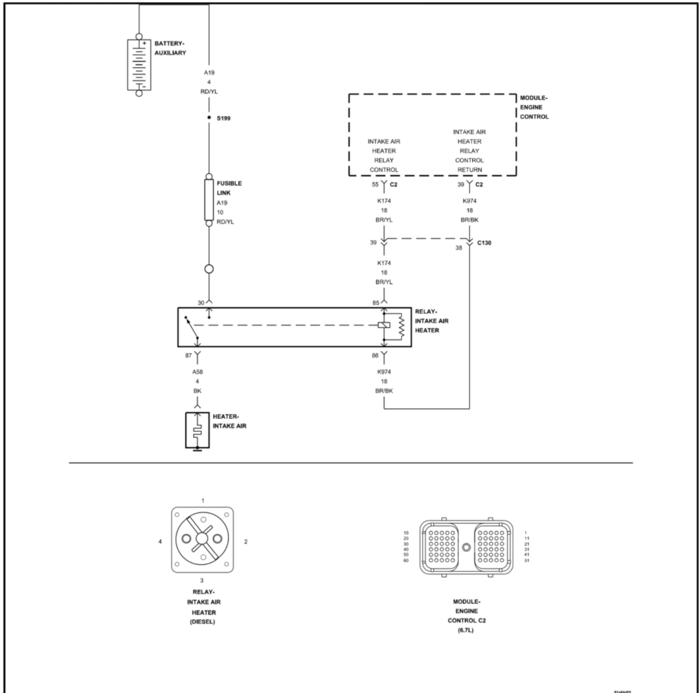
P2609 wiring diagram
