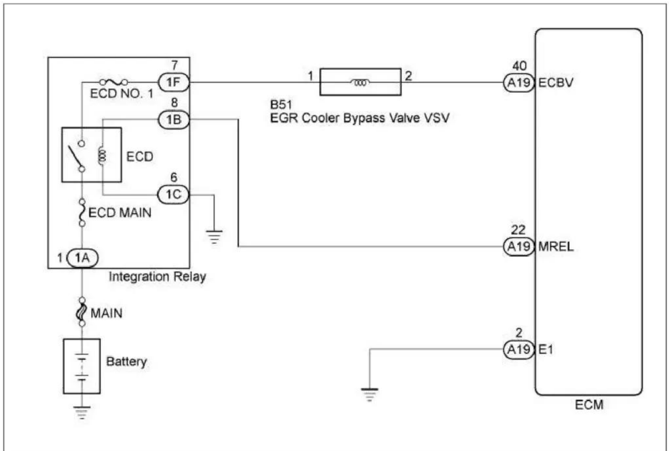
P245D wiring diagram
