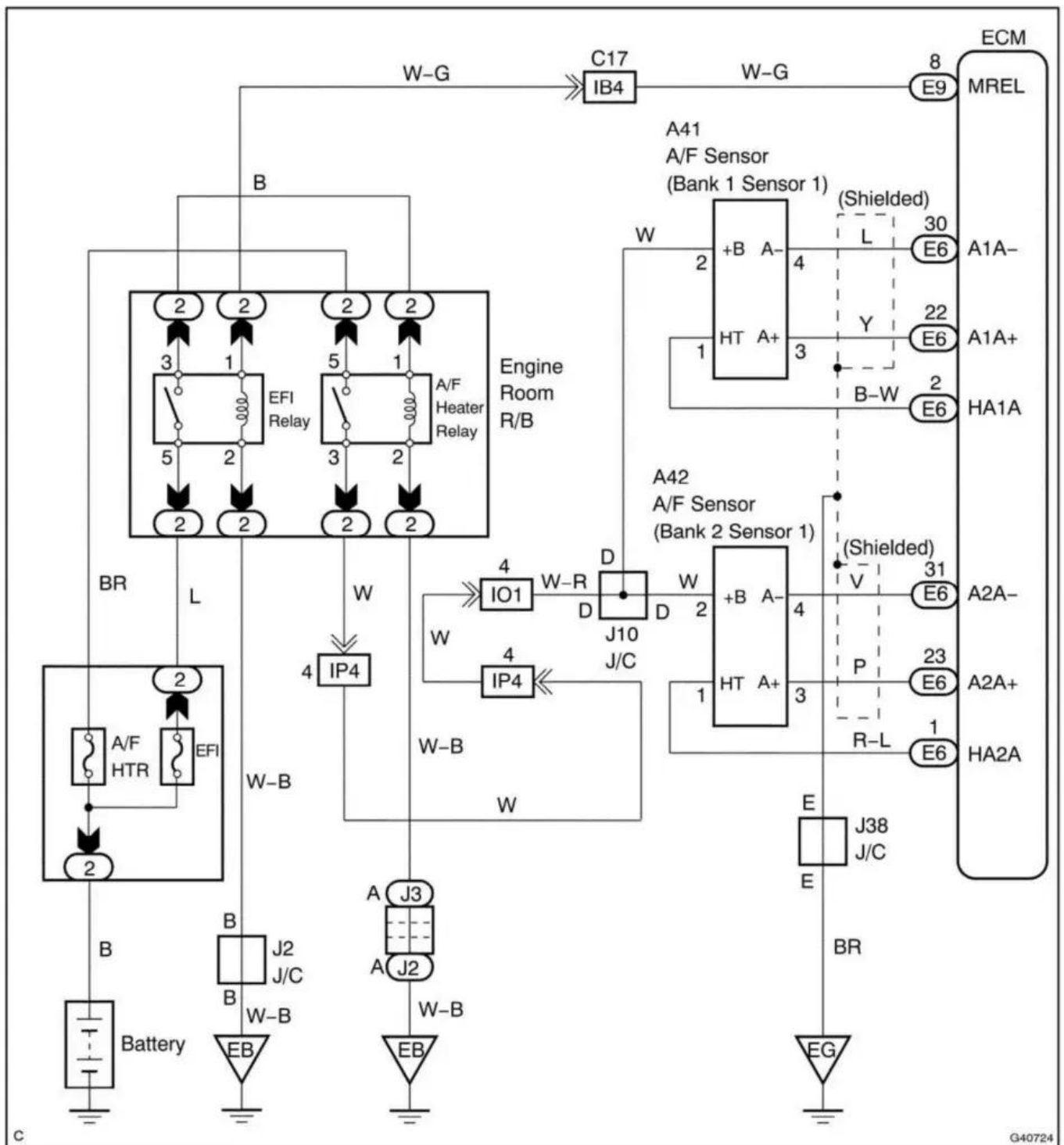
P2195 wiring diagram
