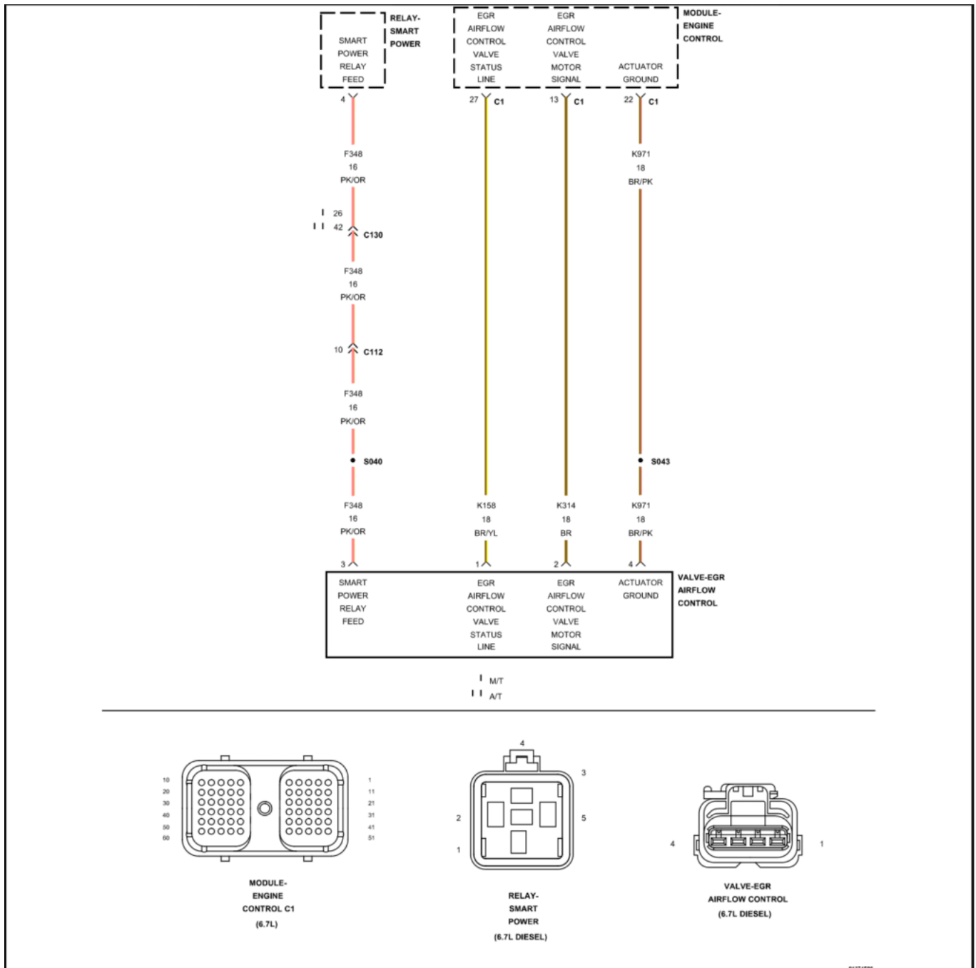
P1241 wiring diagram
