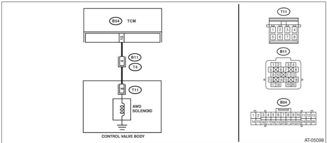
P0971 wiring diagram
