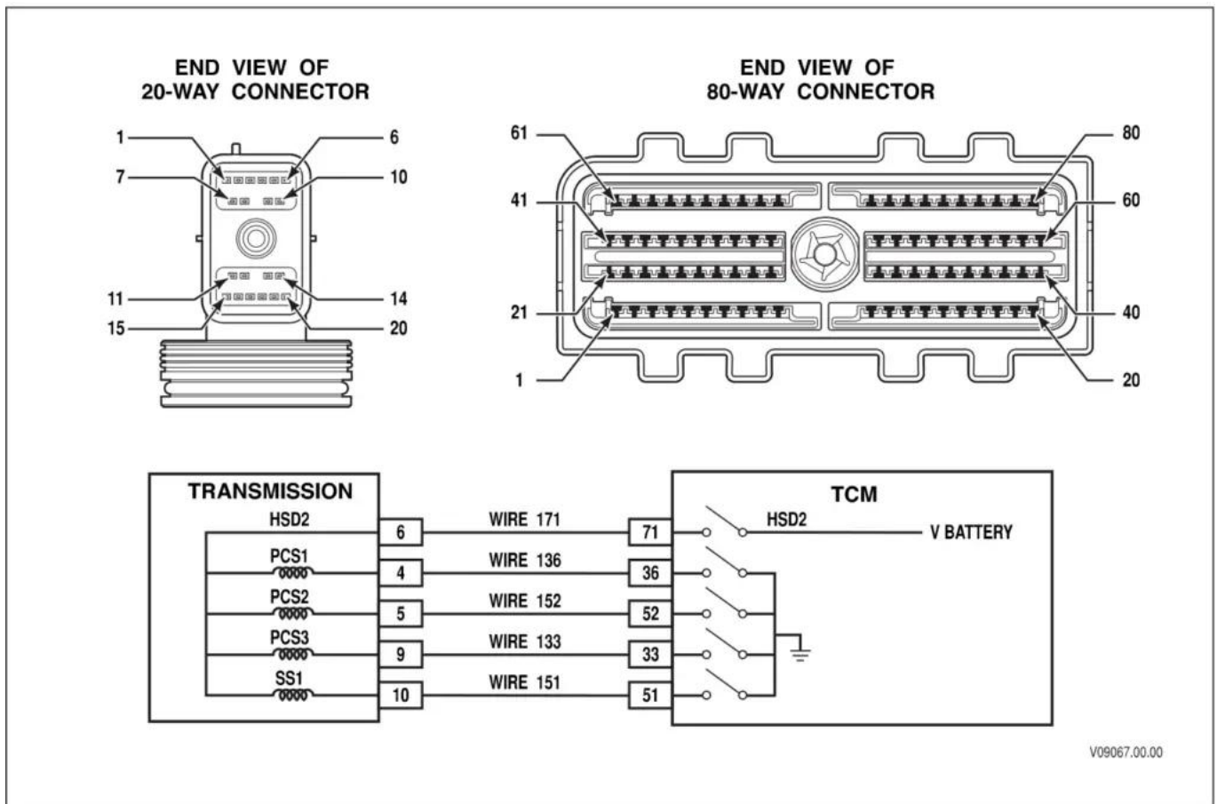
P0967 wiring diagram
