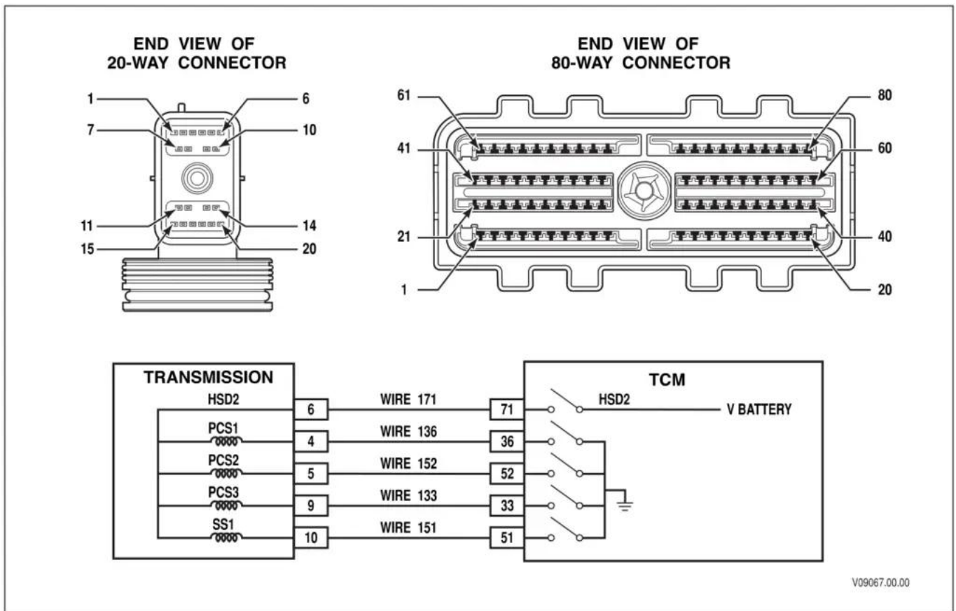
P0964 wiring diagram
