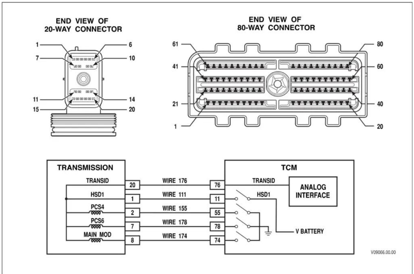
P0963 wiring diagram
