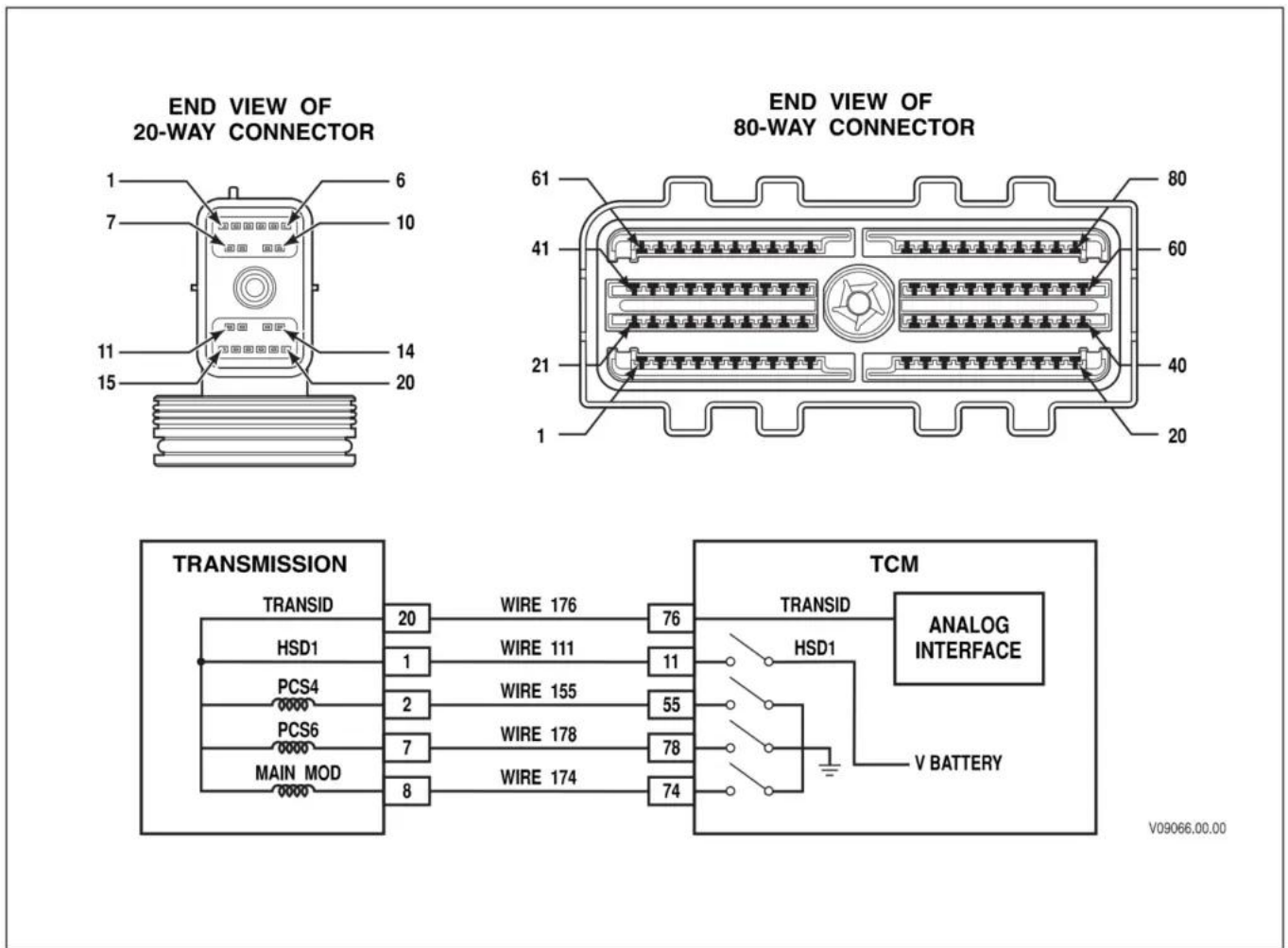
P0960 wiring diagram
