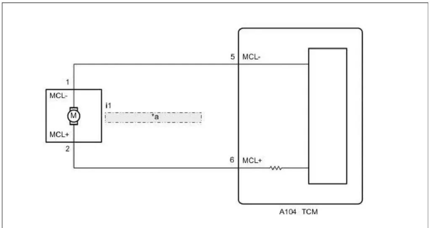
p0900 wiring diagram
