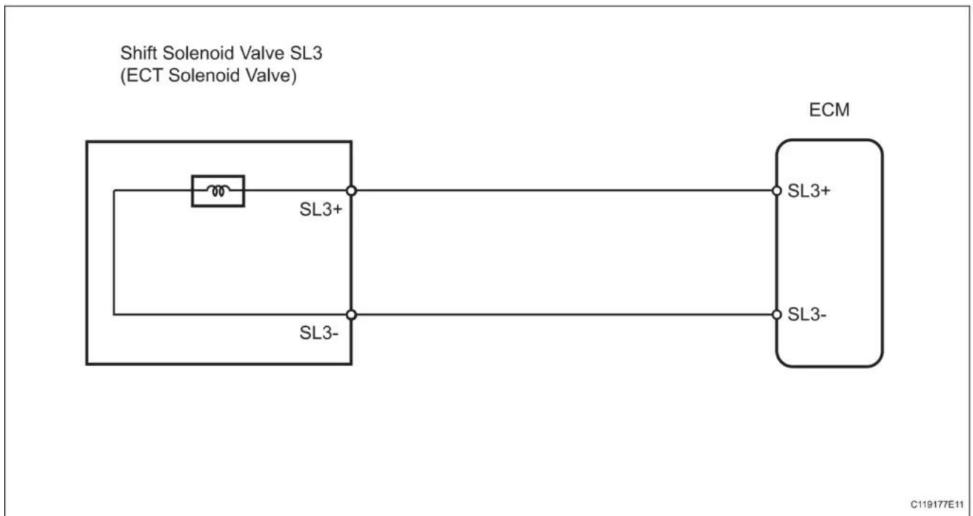
P0798 wiring diagram
