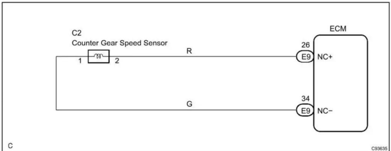
P0793 wiring diagram
