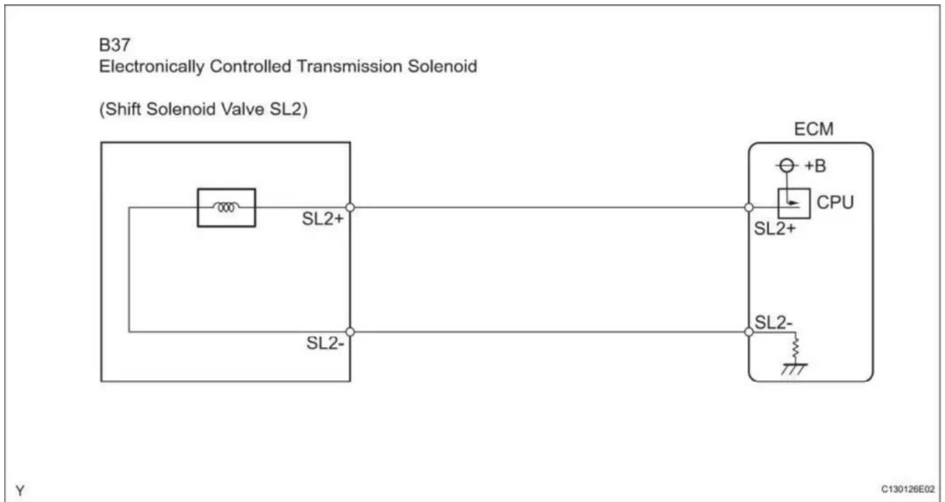
P0778 wiring diagram
