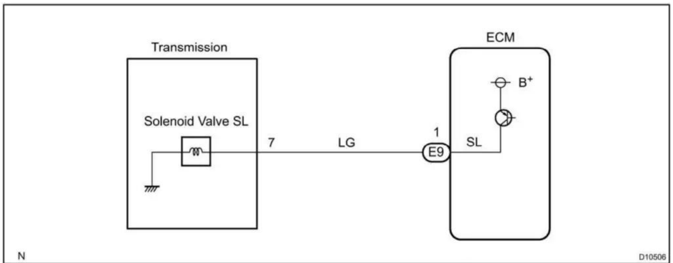
P0773 wiring diagram
