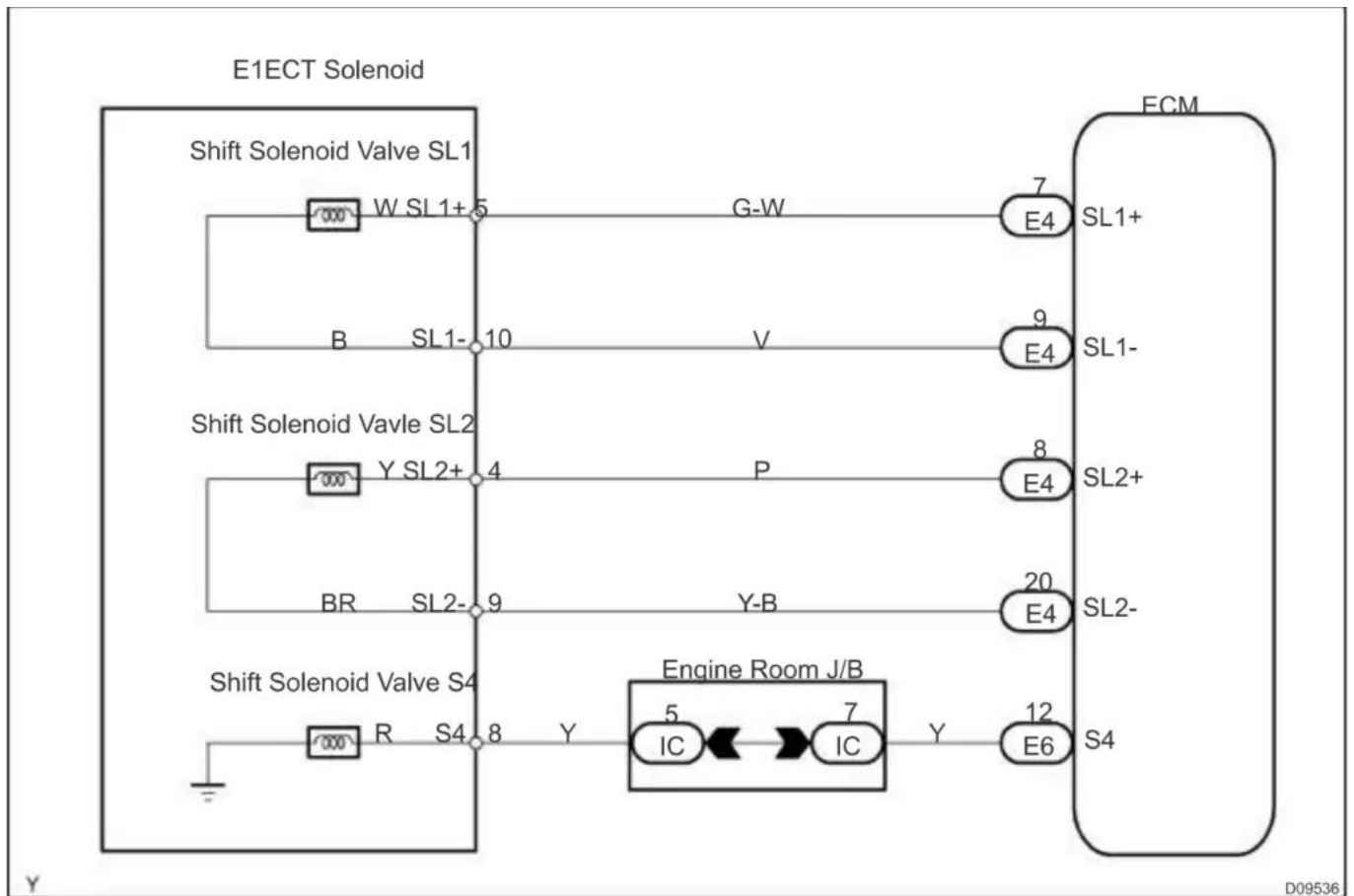
P0768 wiring diagram
