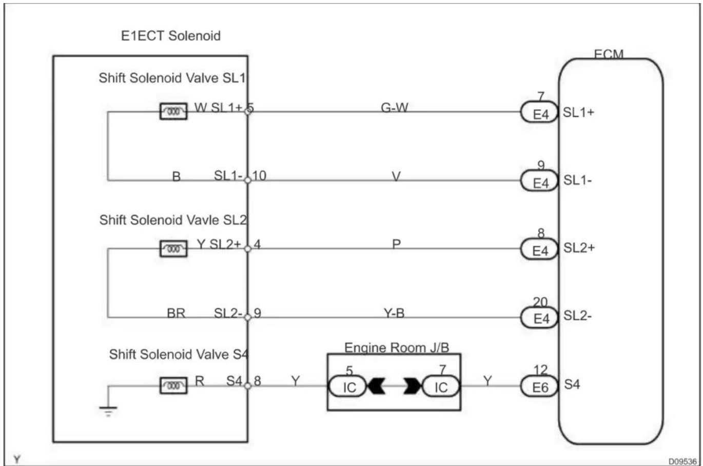
P0758 wiring diagram
