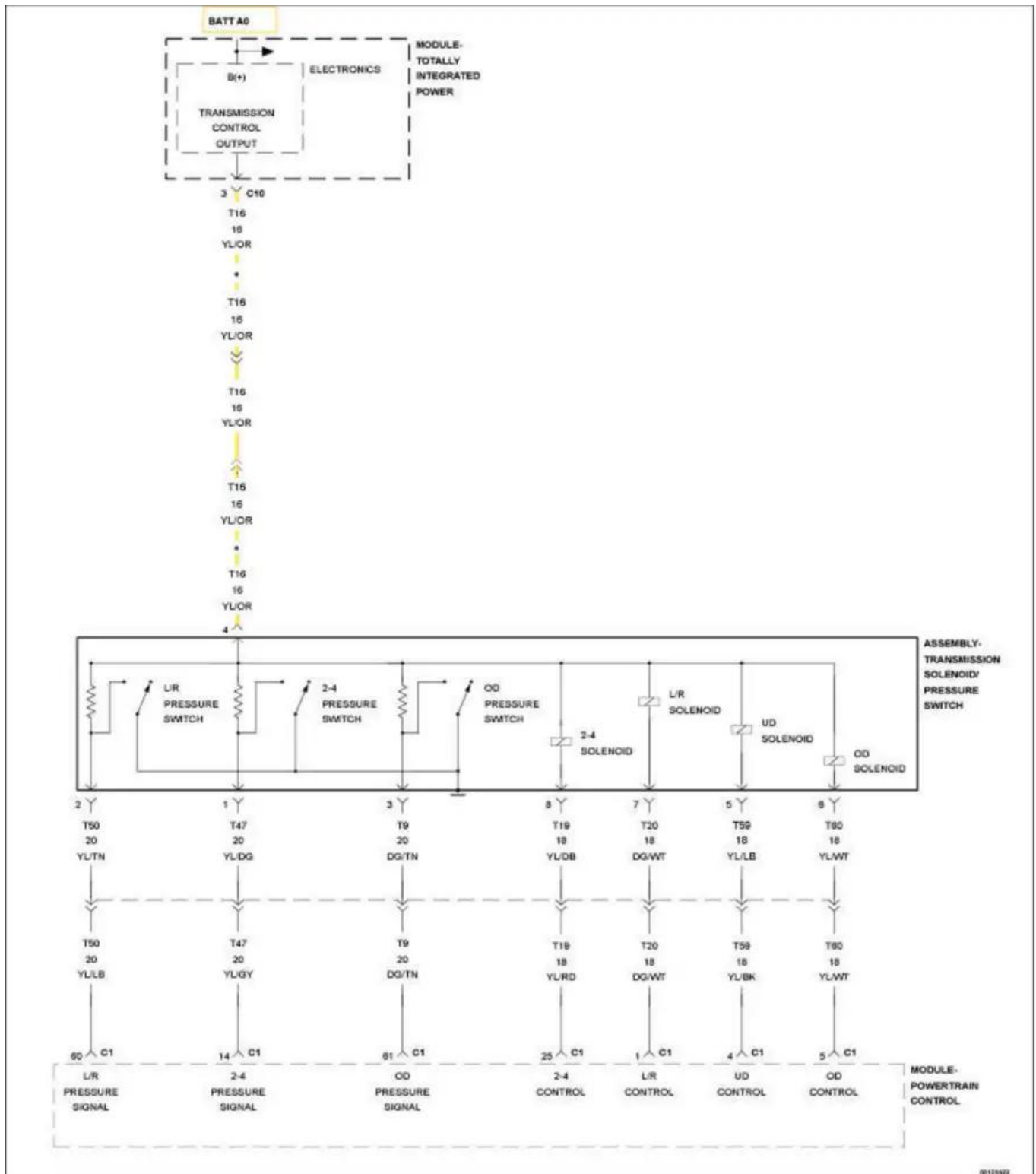
P0755 wiring diagram
