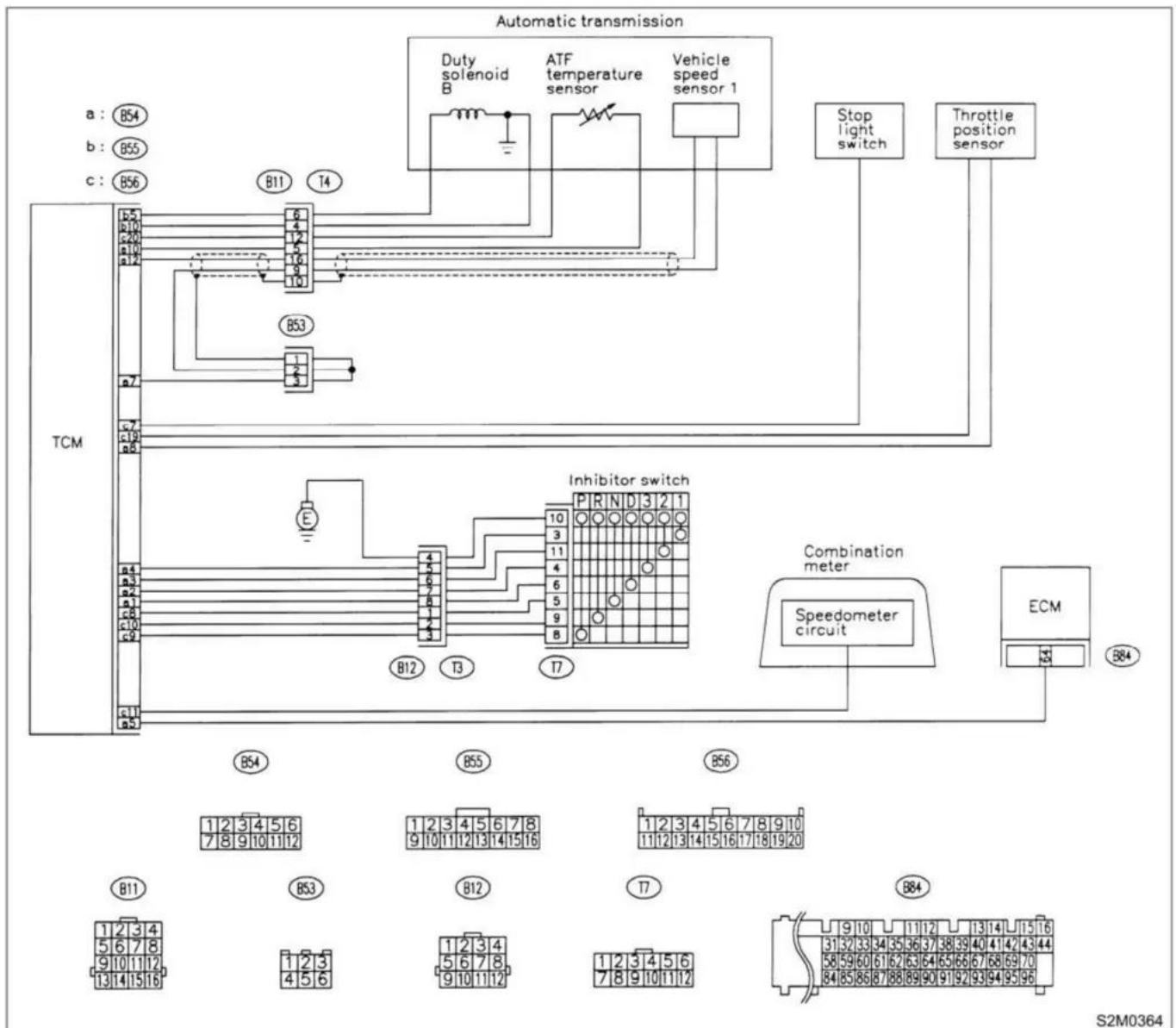
P0740 wiring diagram
