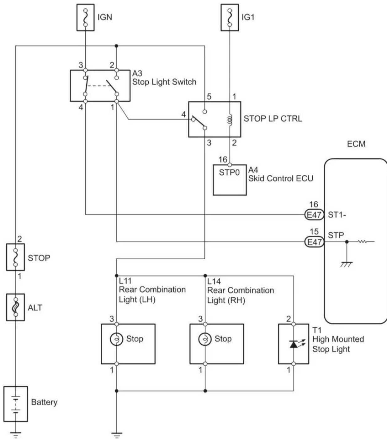
P0724 wiring diagram
