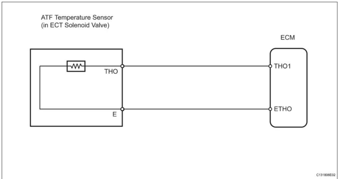
P0713 wiring diagram
