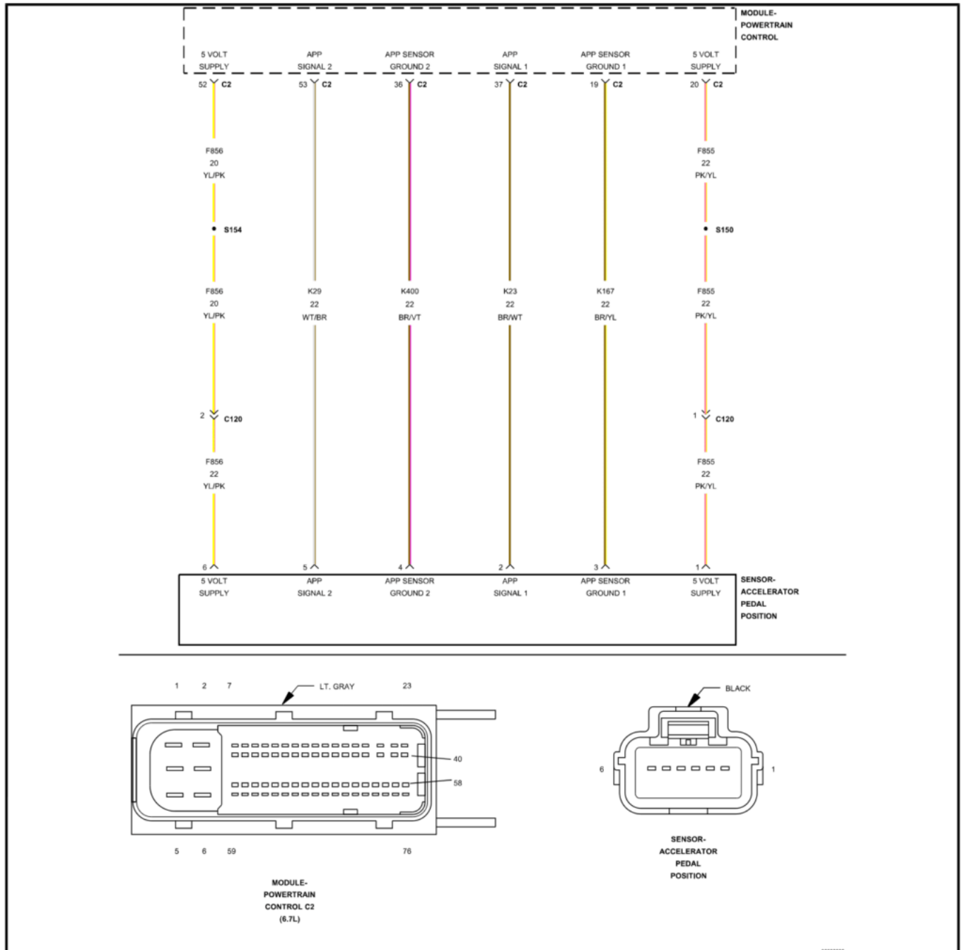
P06A4 wiring diagram
