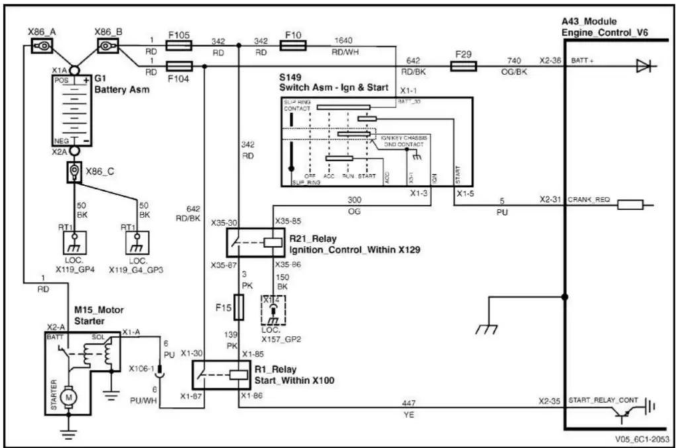
P0617 wiring diagram
