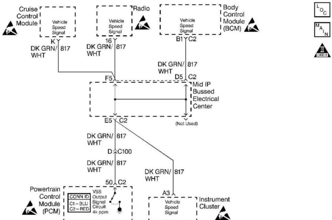
P0608 wiring diagram
