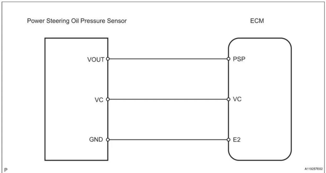
P0550 wiring diagram
