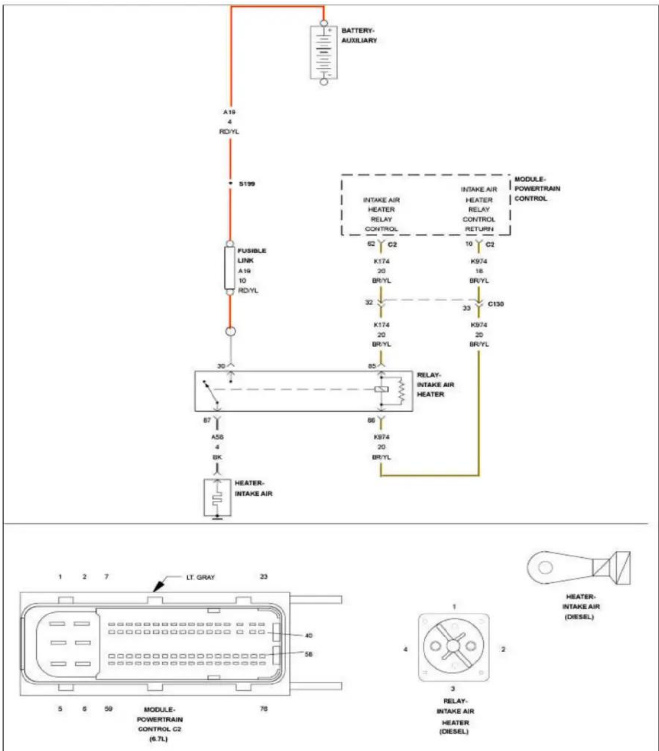
P0542 wiring diagram
