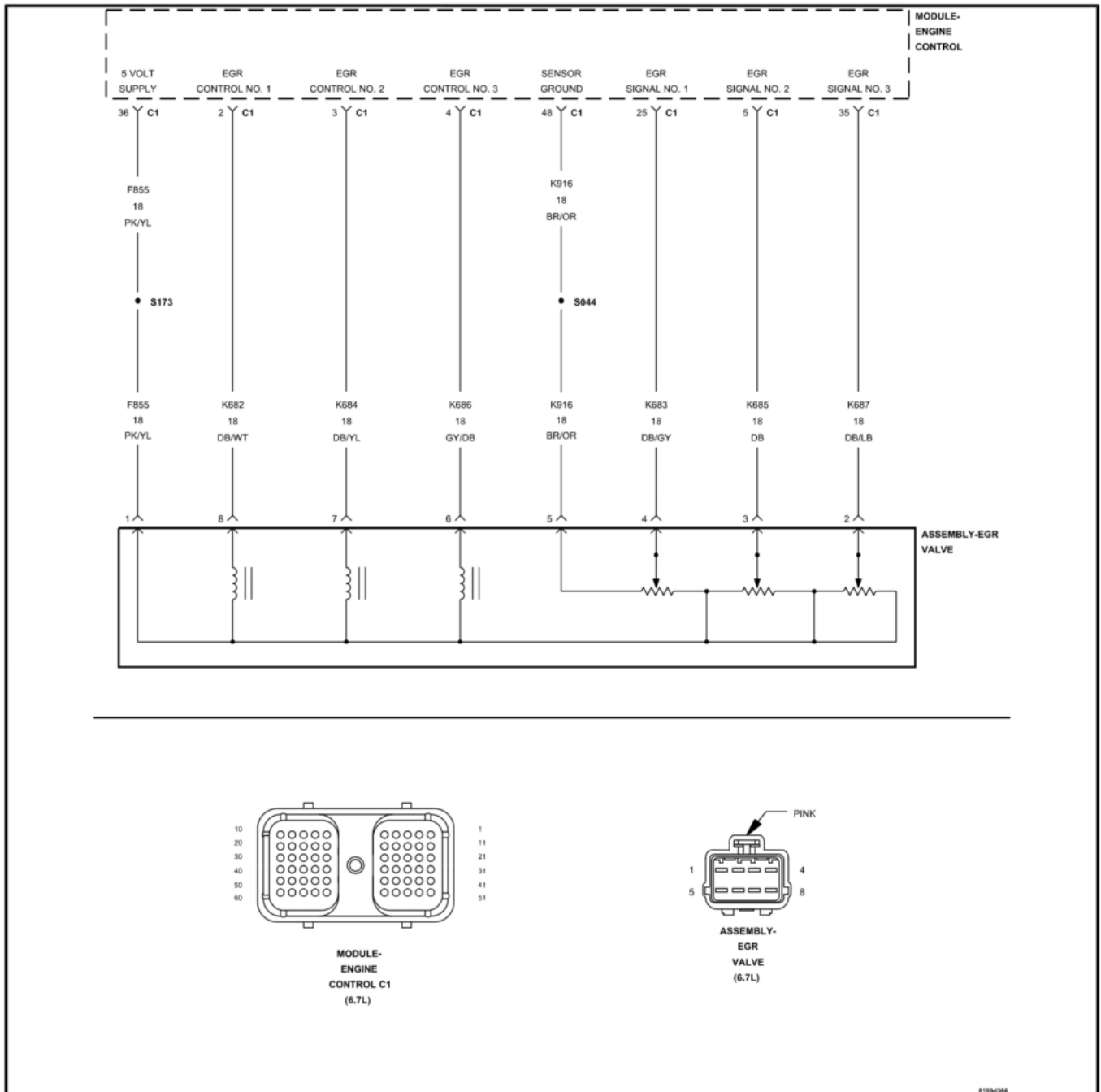
P0489 wiring diagram
