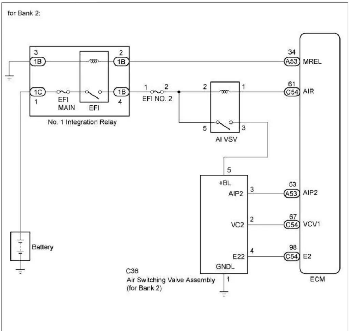
P0417 wiring diagram
