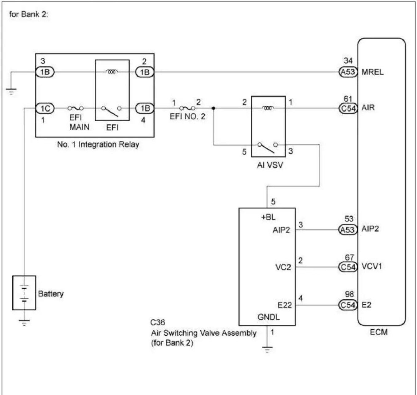
P0416 wiring diagram
