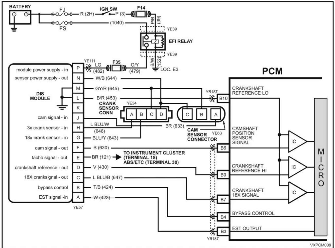
P0374 wiring diagram
