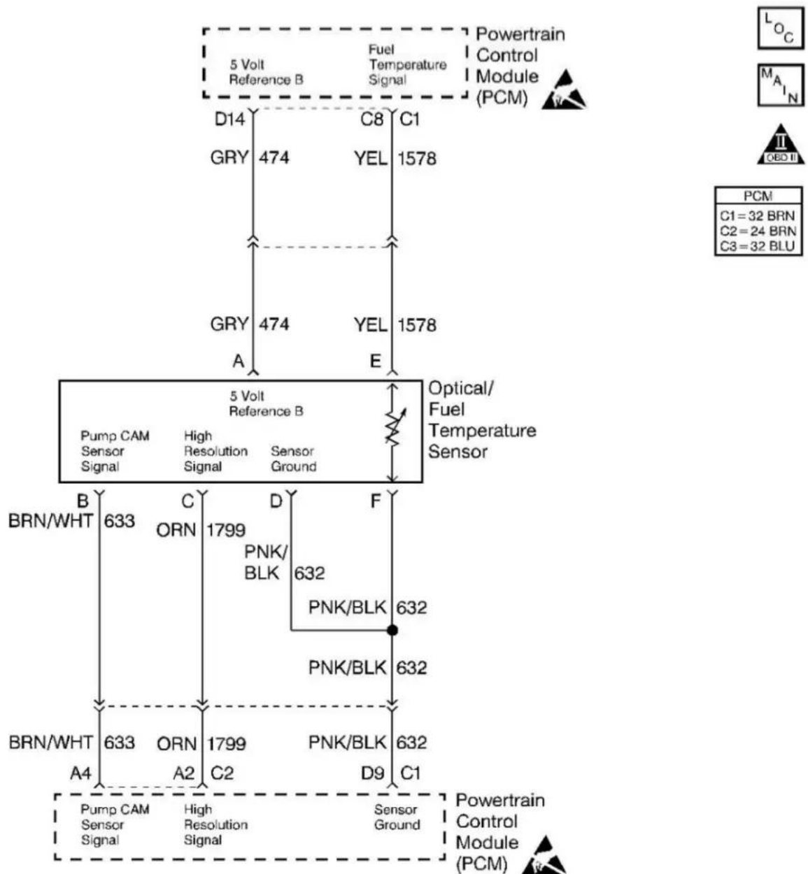
P0370 wiring diagram
