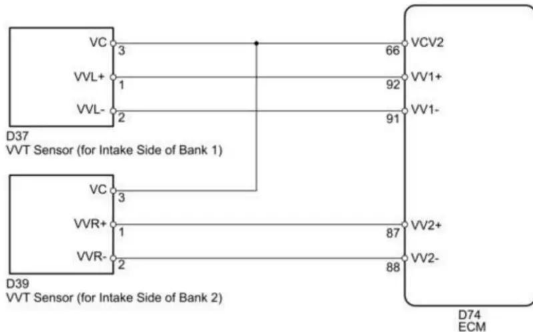
P0343 wiring diagram
