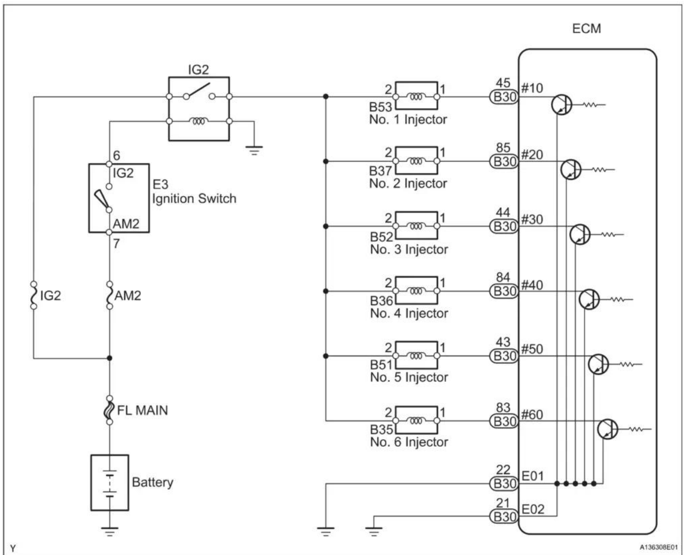
P0304 wiring diagram
