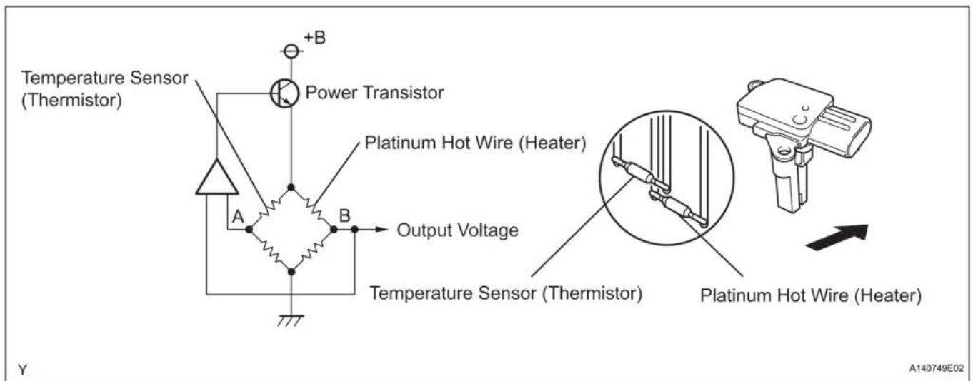
P0101 wiring diagram
