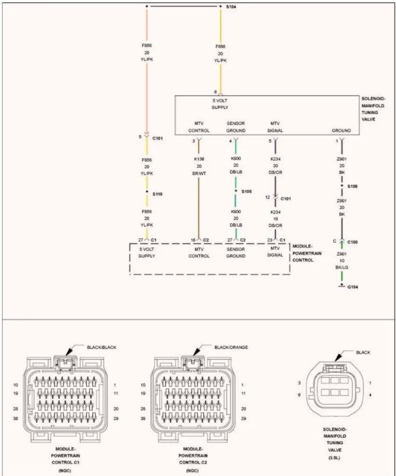
P1005 Dodge wiring diagram
